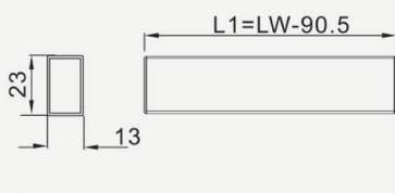
Aluminum front rail
