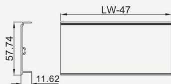
Inner drawer aluminum front panel cover
